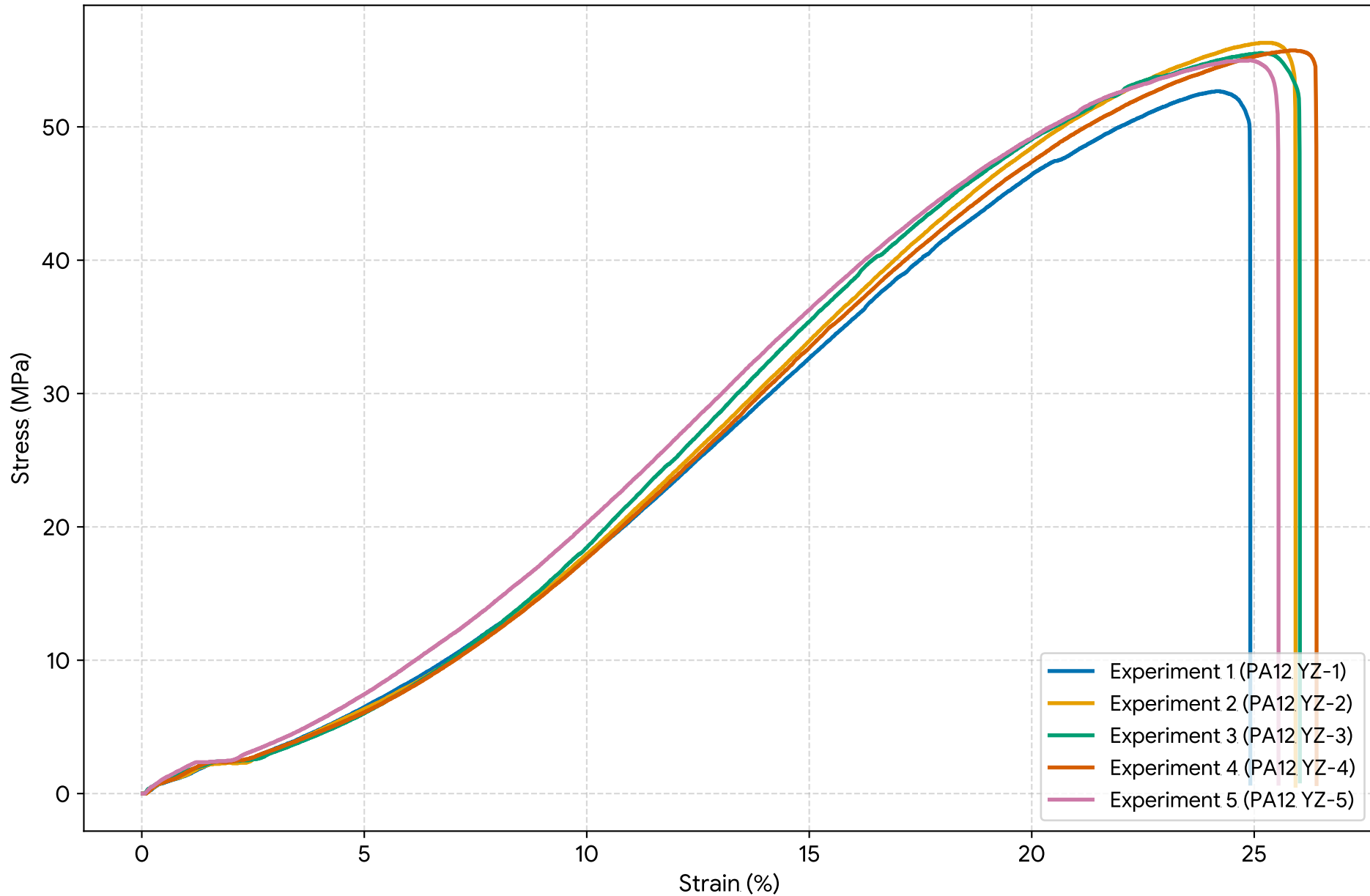
Stress-Strain Curves for PA12 YZ (5 Experiments)
